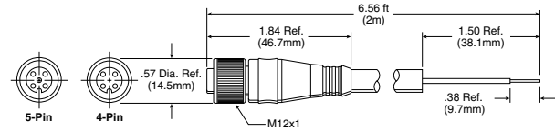
Female Interface 5-Pin, M12
